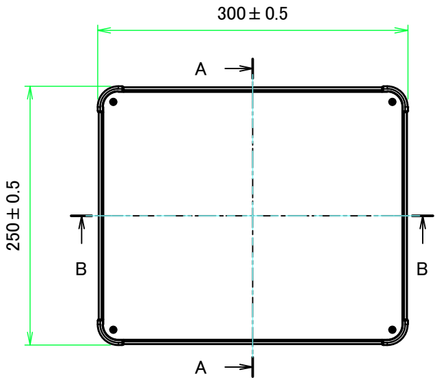
E view
