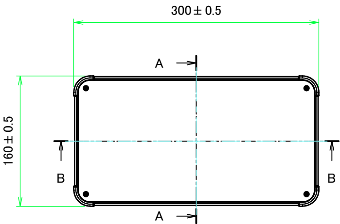
E view
