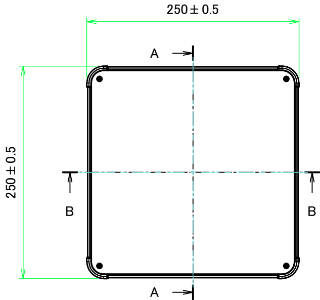
E view
