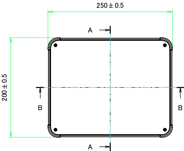
E view
