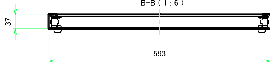
B-B (1:6)
