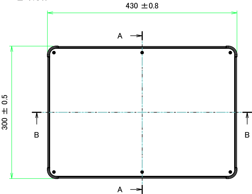
E view
