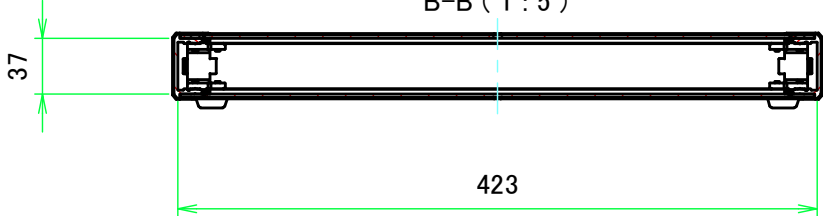
B-B (1:5)
