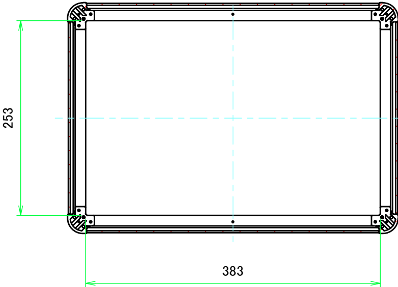
C-C (1:5)
