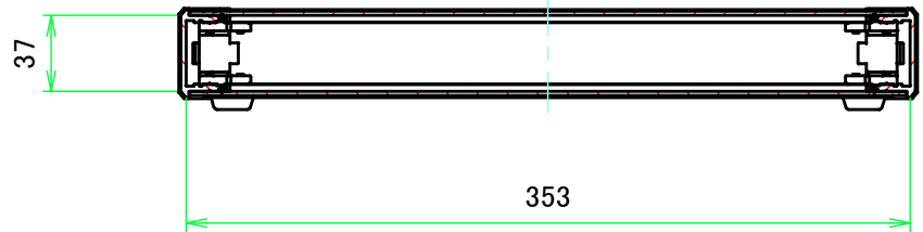
B-B (1:4)
