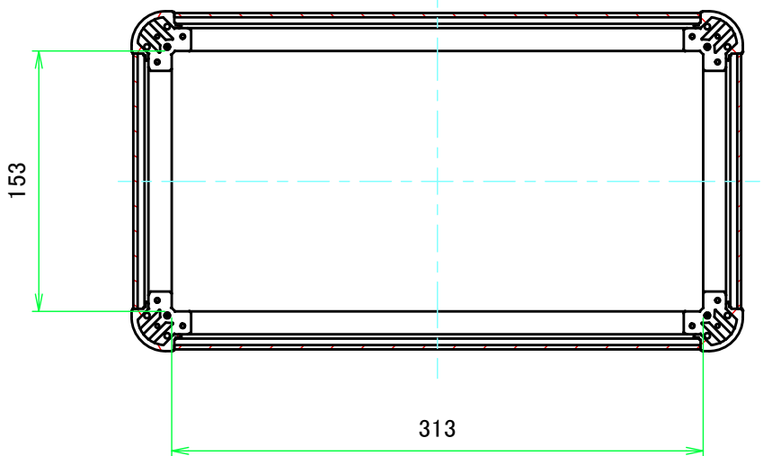
C-C (1:4)
