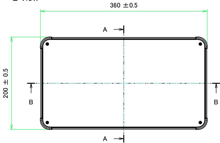
E view
