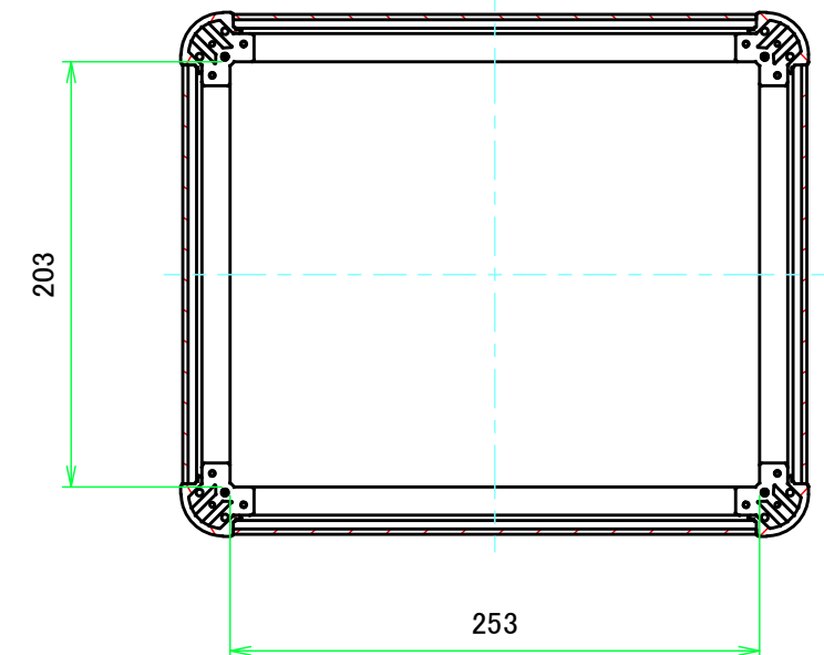
C-C (1:4)
