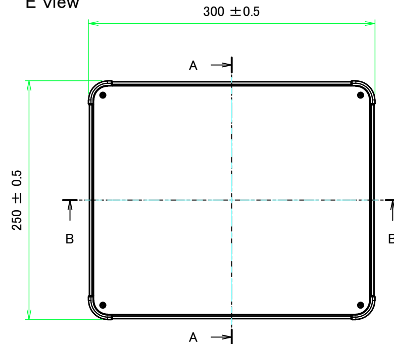
E view
