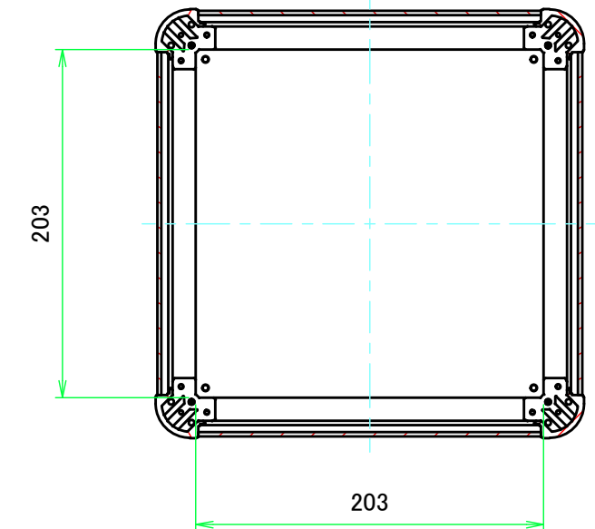
C-C (1:4)
