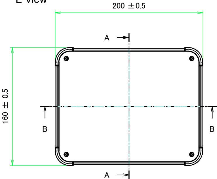
E view
