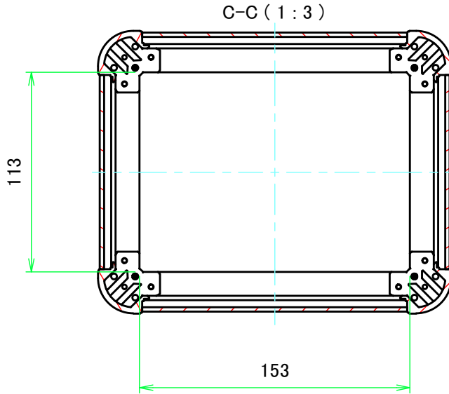
C-C (1:3)
