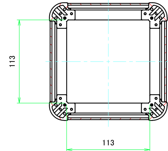
C-C (1:3)
