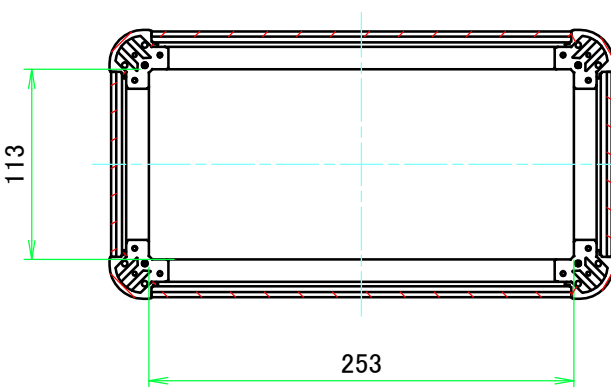
C-C ( 1 :4.5 )
