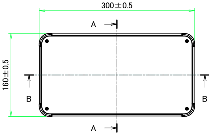
E view
