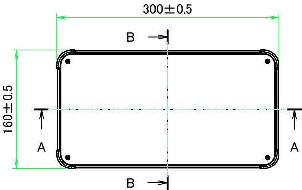
E view
