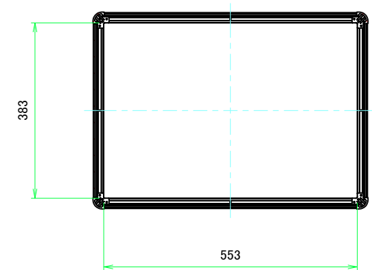
C-C (1:8)
