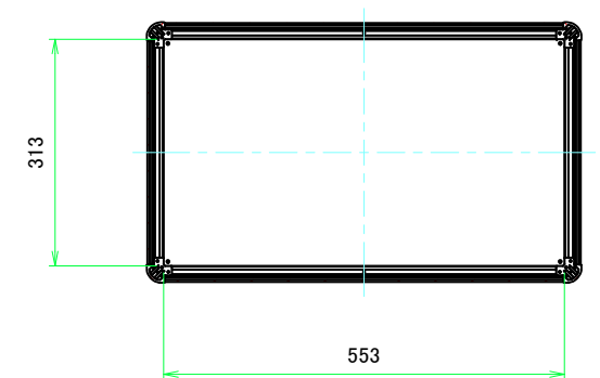
C-C (1:8)
