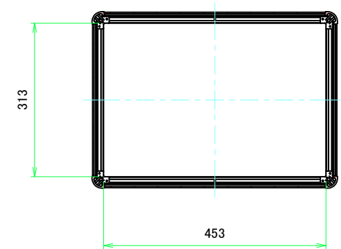
C-C (1:7.5)
