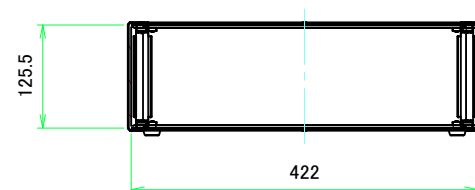
B-B (1:6.5)
