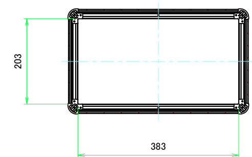
C-C (1:6.5)
