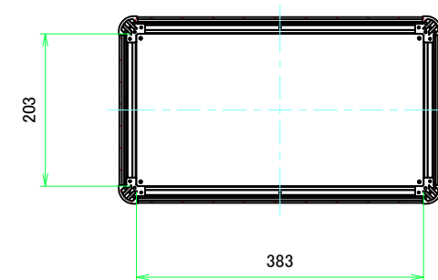
C-C (1:6.5)
