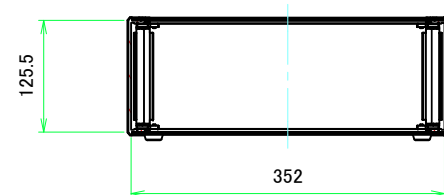
B-B (1:6)
