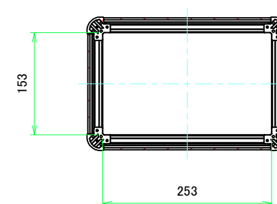
C-C (1:5.5)
