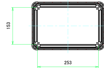
C-C (1:5.5)
