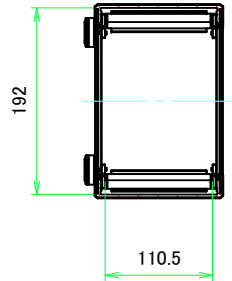
A-A (1:5.5)
