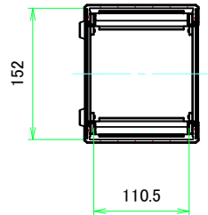
A-A (1:5.5)
