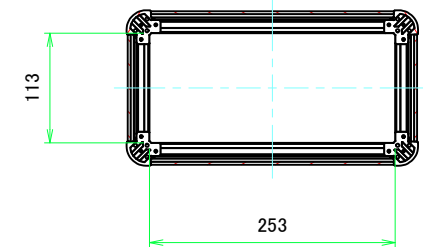
C-C (1:5.5)
