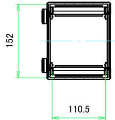
A-A (1:5.5)
