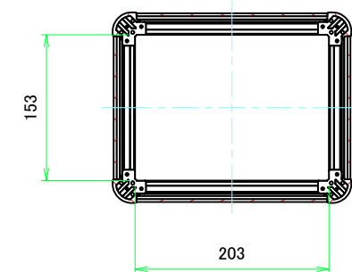
C-C (1:5)
