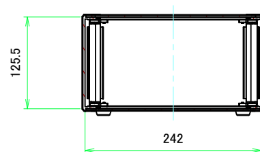
B-B (1:5)
