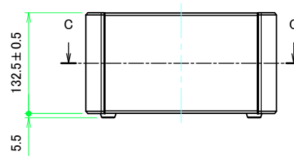
A view
