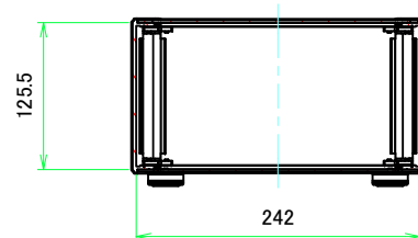
B-B (1:5)
