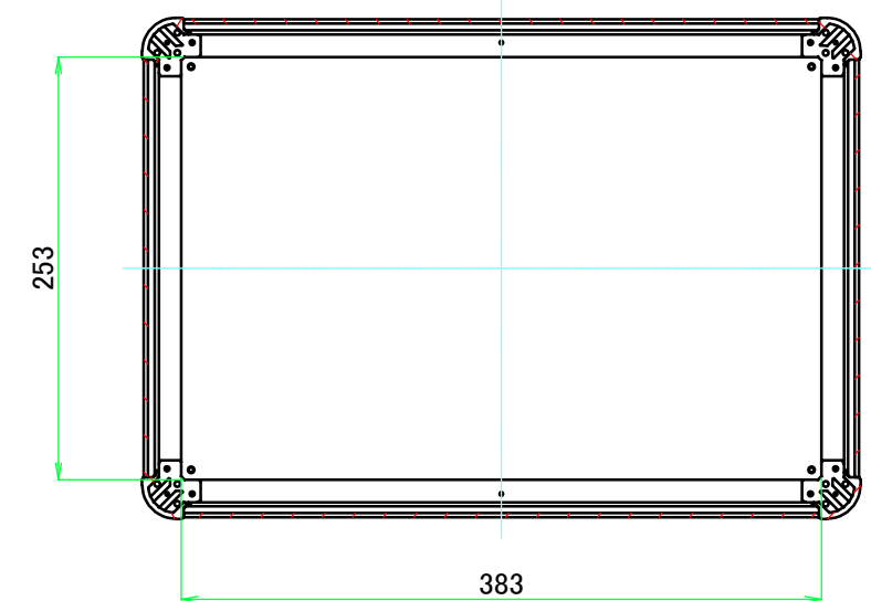
C-C (1:5)
