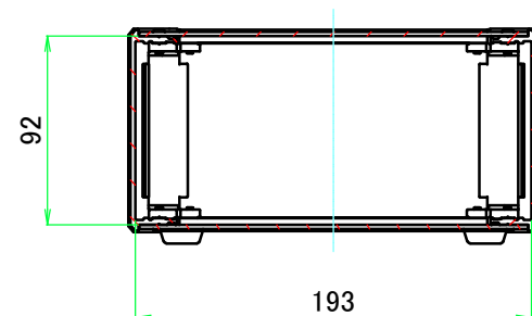
B-B (1:4)
