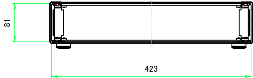
B-B (1:5)
