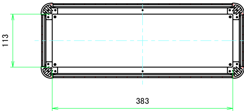
C-C (1:5)
