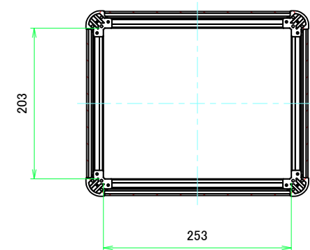
C-C (1:5)
