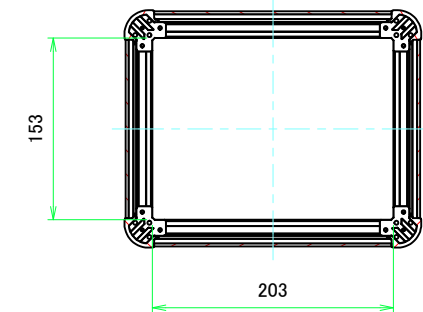
C-C (1:4.5)
