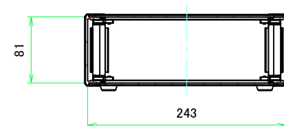
B-B (1:4.5)
