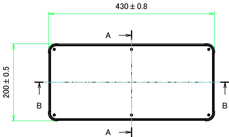
E view
