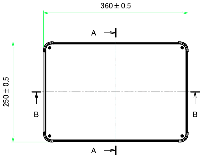
E view
