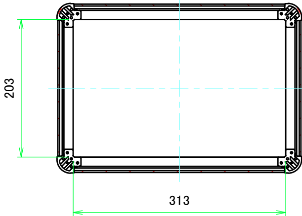
C-C ( 1:5.5 )
