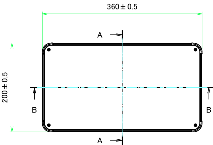
E view
