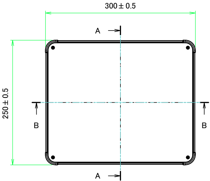
E view
