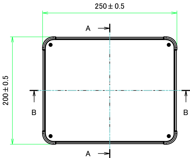
E view
