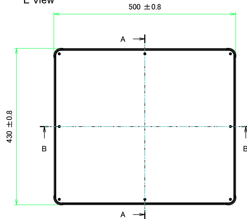
E view
