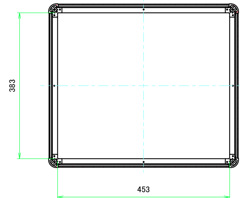
C-C (1:6)
