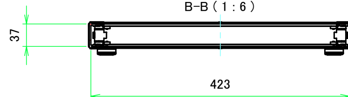
B-B (1:6)
