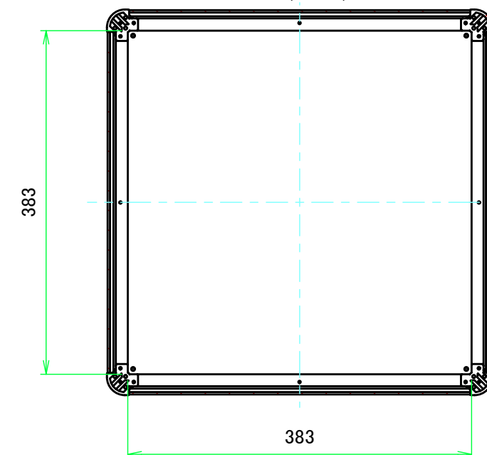
C-C (1:6)
