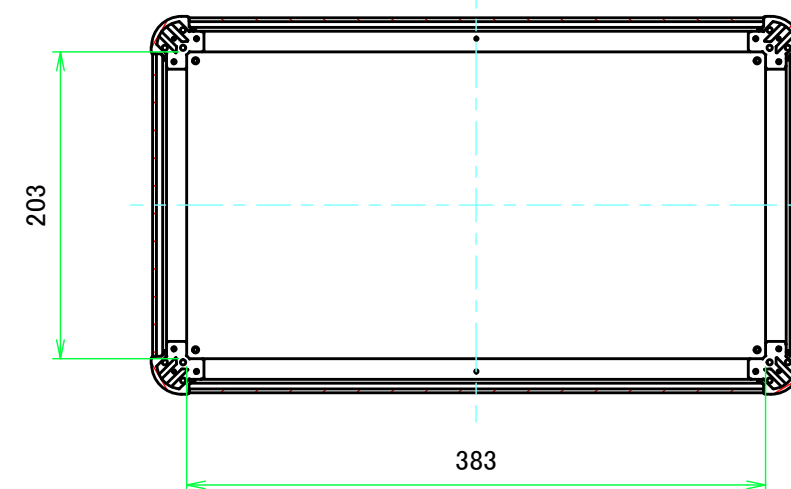
C-C (1:5)
