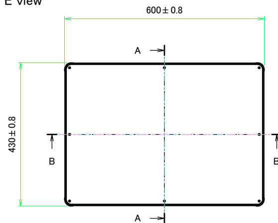
E view
