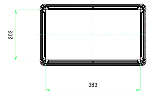
C-C (1:6.5)
