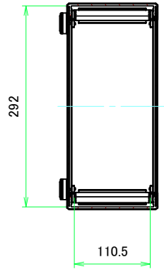
A-A (1:5.5)
