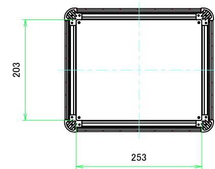
C-C (1:5.5)
