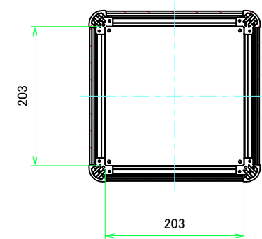
C-C (1:5.5)
