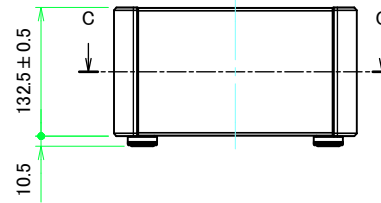
B-B (1:5.5)
