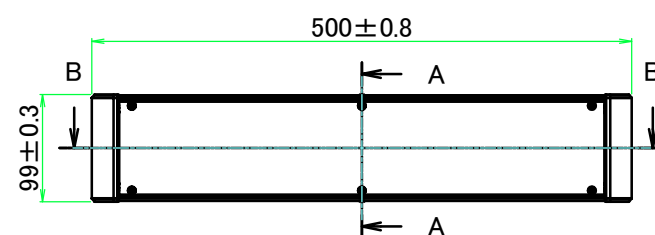
A view
