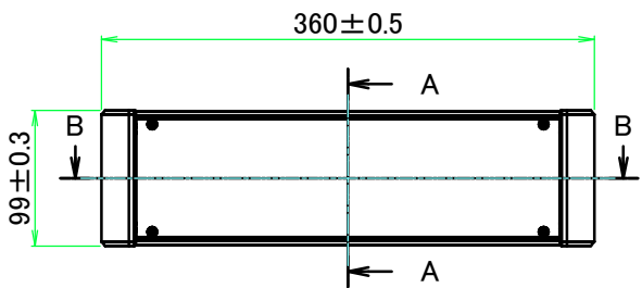
A view
