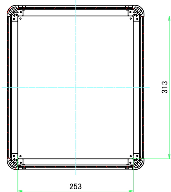
B-B (1:5)
