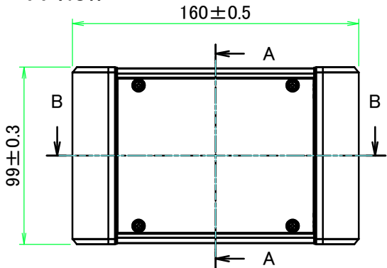
A view
