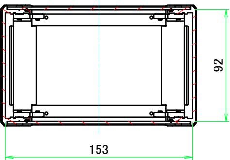
C-C (1:3)
