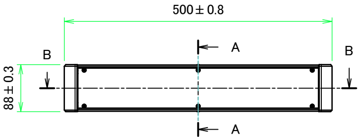
A view
