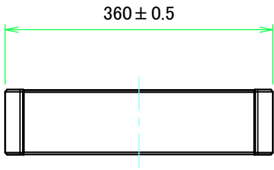
C view
